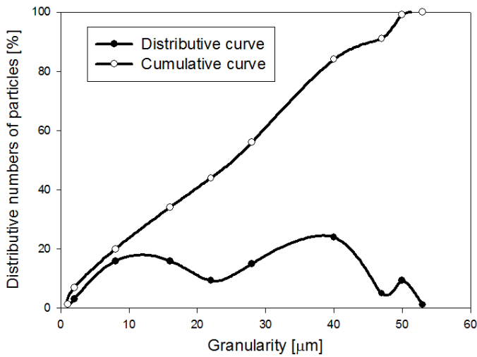
Fig. 2. Granulometric distribution of EAFD sample
