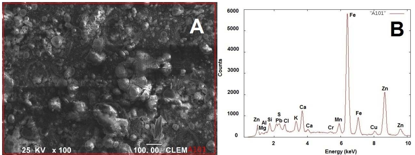
Fig. 3. (A) SEM image of EAFD sample, (B) EDS analysis of EAFD sample
