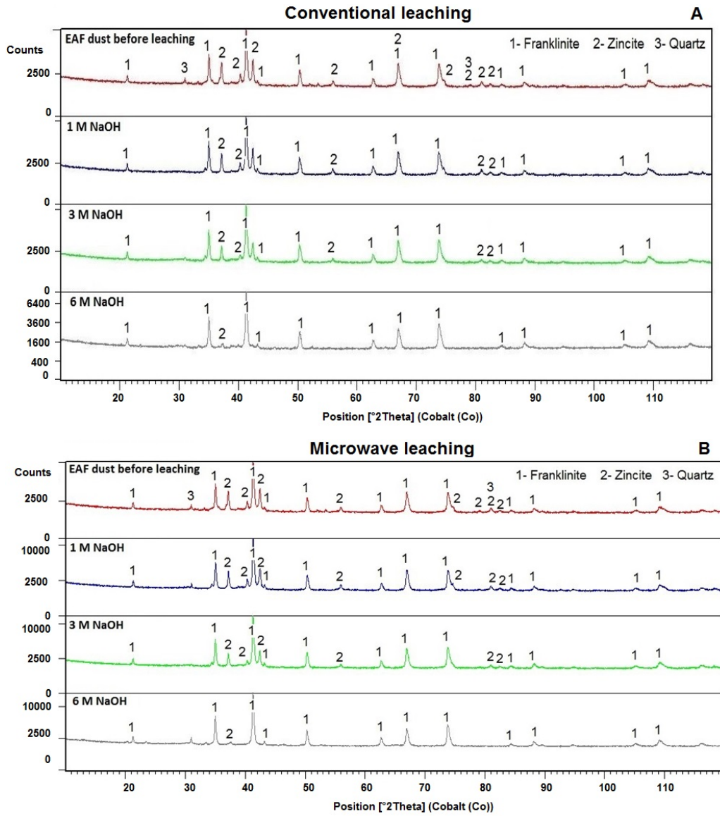
Fig. 9. Comparison of XRD patterns of different leaching residues after (A) conventional leaching and (B) MW-assisted leaching
